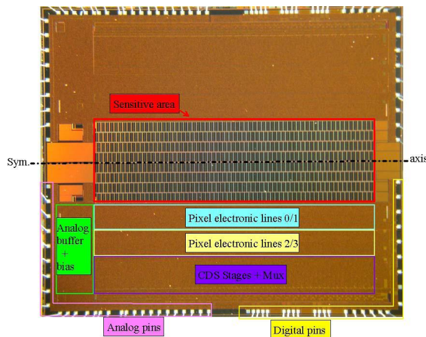
Figure 8: UserCams electronic sensor
