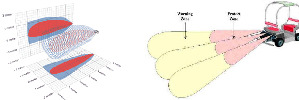
Figure 1: The Ultrasonic shape (left) and the two zones (right)
