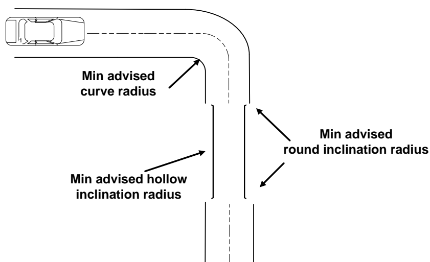
Figure 12. Predefined test course
