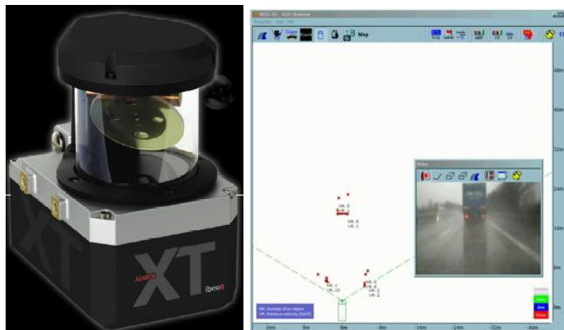
Figure 4: the IBEO XT Alasca and an illustration of this system with rain
