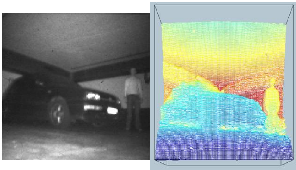
Figure 7: Output of a Swissranger 3D camera
